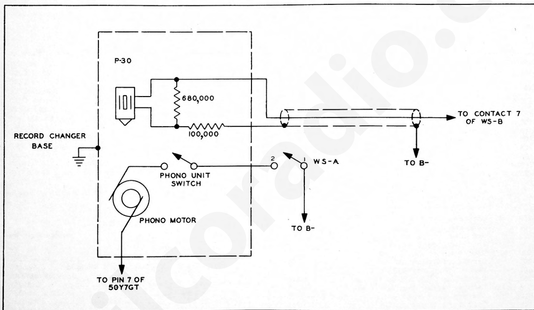
Wiring Diagram of Record Changer (M-9) in Model 49-1404
